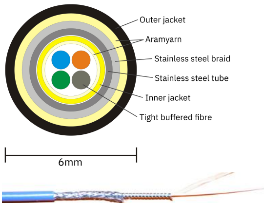
Round Micro Armoured Fibre Patch Cable
